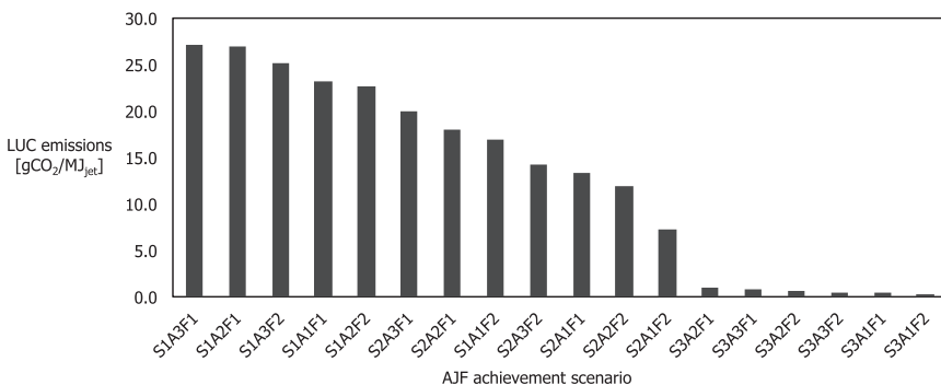
Fig. 6. LUC emissions [gCO 2 /MJ jet ] averaged over AJF from all cultivated energy crops, by AJF scenario.
