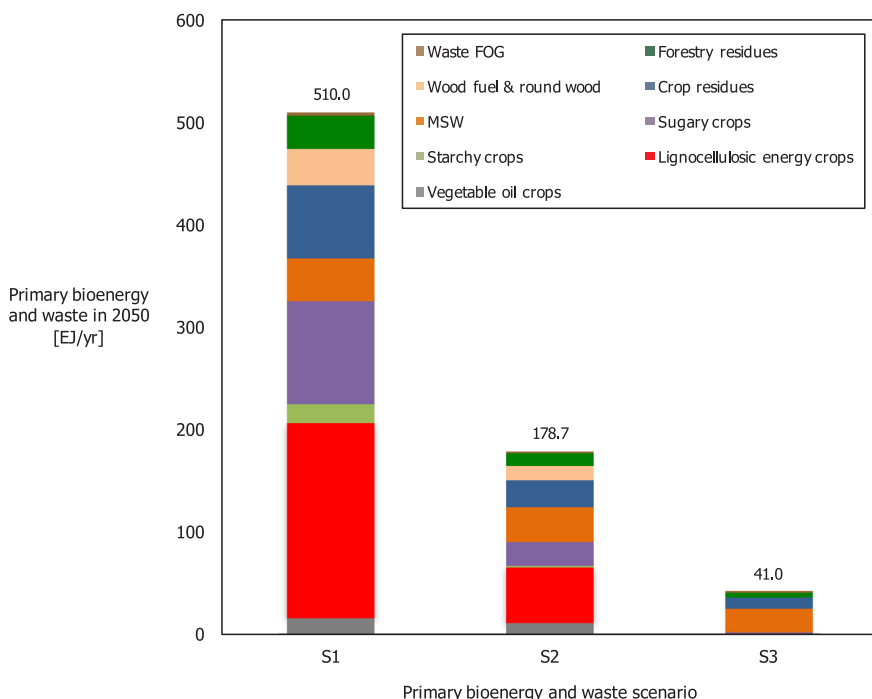
Fig. 2. 2050 primary bioenergy and waste results, broken out by feedstock type. Note that microalgae is not included at this step of the analysis.
