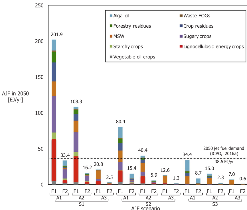
Fig. 5. AJF scenario results, compared to projected 2050 jet fuel demand (ICAO, 2016a).
