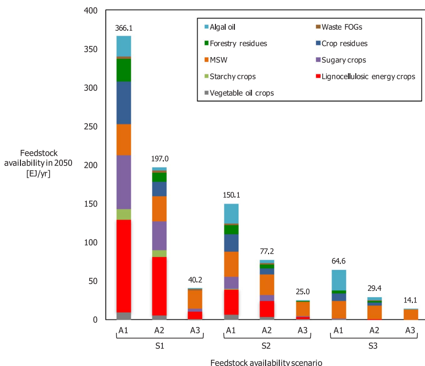
Fig. 4. 2050 feedstock availability results.
