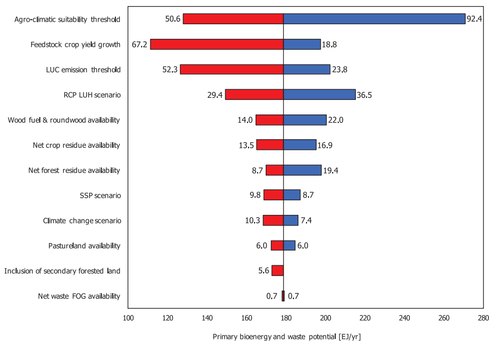
Fig. 3. S2 results' (178.7 EJ/yr) sensitivity to 2050 primary bioenergy and waste scenario assumptions. Scenario and sensitivity parameter definitions are found in Table S34 of the SI.
